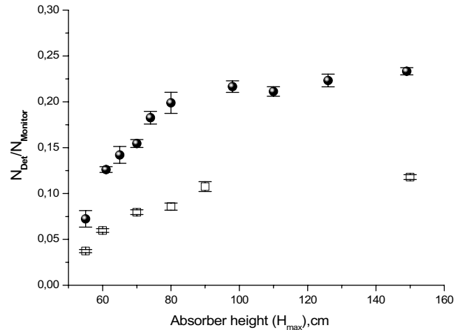
Fig. 11. Plot of measurement results with a powder of diamond nanoparticles: the number of VUCN as a function of maximum absorber height, normalized to the number of monitor counts (per main part of the measurement cycle). The black circles correspond to the measurement at room temperature. The white squares indicate measurement at 108 K.
